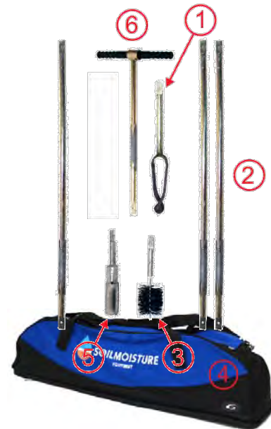
Fig. 5. Model 0237D10L10 components.
