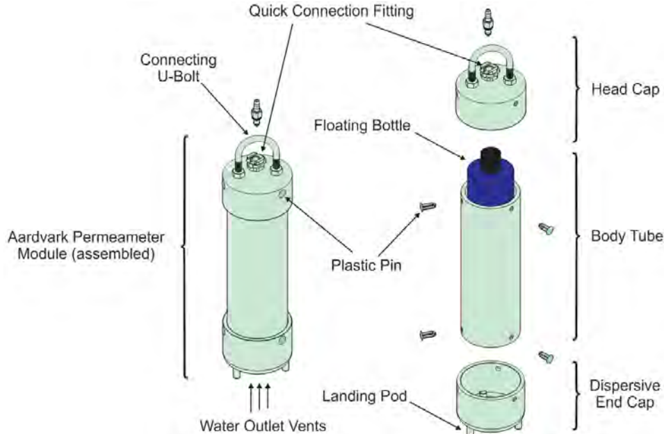
Fig. 7. Left: assembled Aardvark Permeameter Unit. Right: Major Components of APM.
